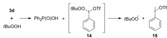
Scheme 2. Proposed pathway for the formation of iodanyl radical.
